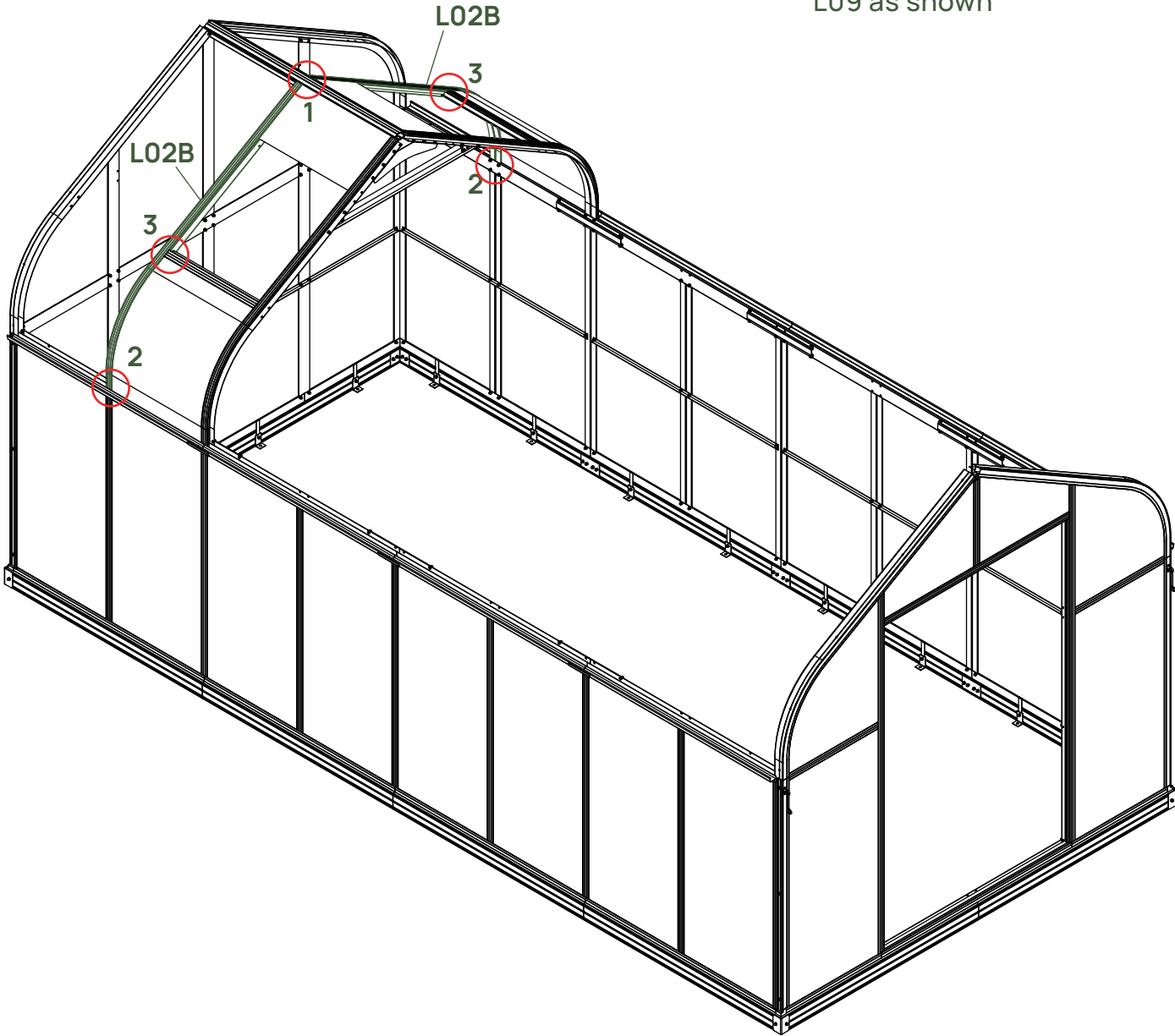
Insert the cut end of L02B onto L09 as shown
